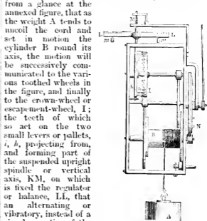
Fig. 1.—De Wyck's Clock.
